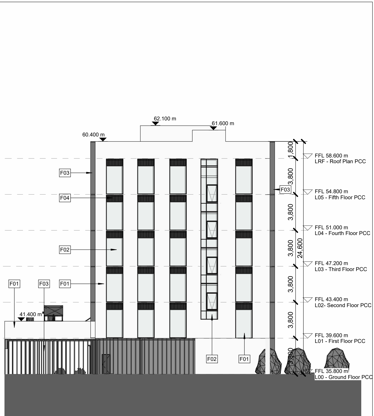
East Elevation PCC 1 : 200
