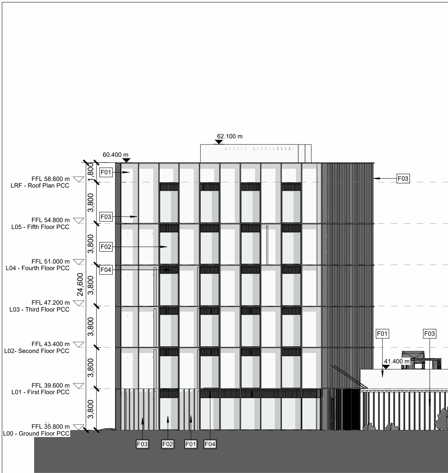
West Elevation PCC 1 : 200
