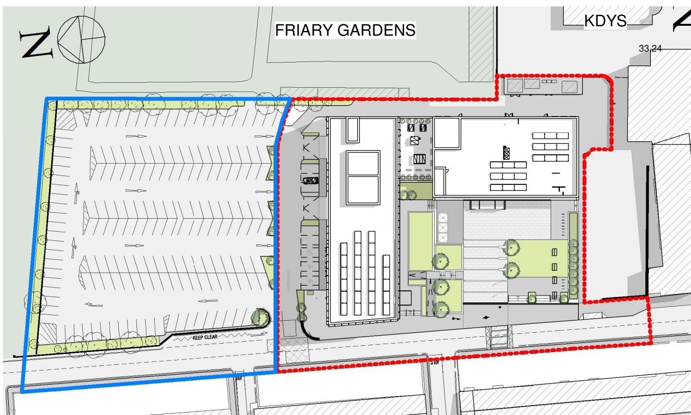
Site Plan - Sun Study 12noon summer 1 : 1000
