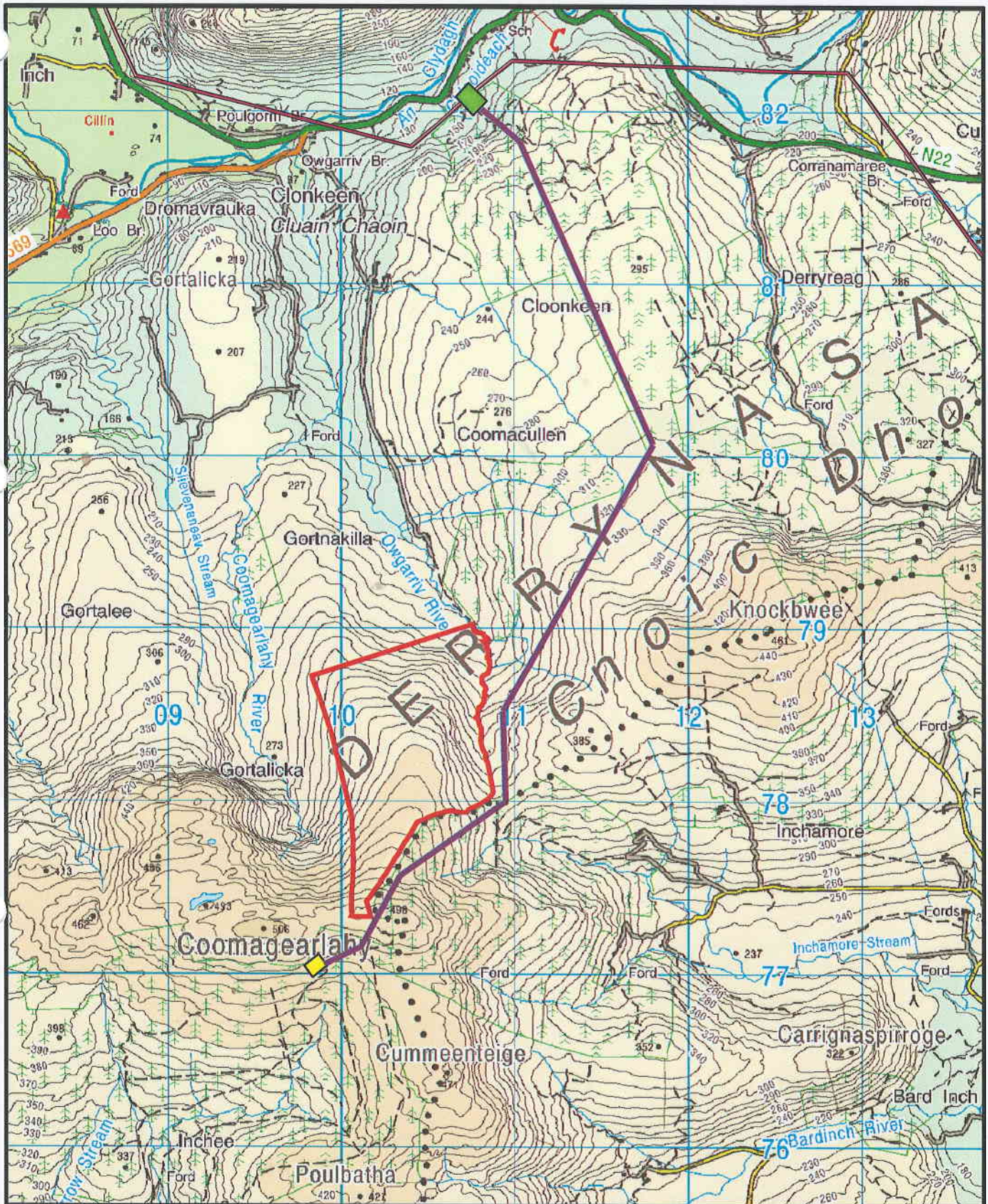
Figure 2.2 Grid Connection Route
